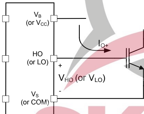
Figure 1: HVIC sourcing current
